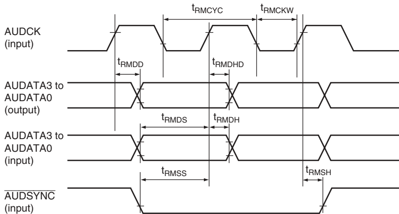
Figure 25.28 RAM Monitor Timing
