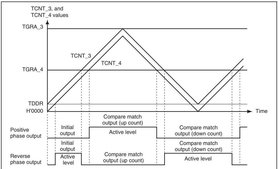
Figure 10.2 Complementary PWM Mode Output Level Example
